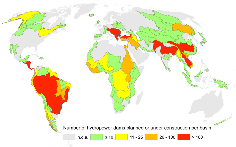
Fig. 3 Number of future hydropower dams per major river basin. Red >100, Orange 26–100, Yellow 11–25, Green ≤10, Gray no data available
