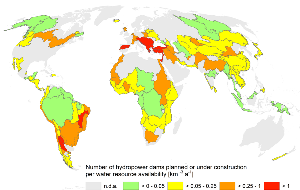
Fig. 4 Number of future hydropower dams in relation to major river basin discharge (dams per \text{km}^3 \text{ year}^{-1} ). Red >1, Orange >0.25–1, Yellow >0.05–0.25, Green >0–0.05, Gray no data available. For comparison with existing hydropower dams please see Online Resource Fig. S10
